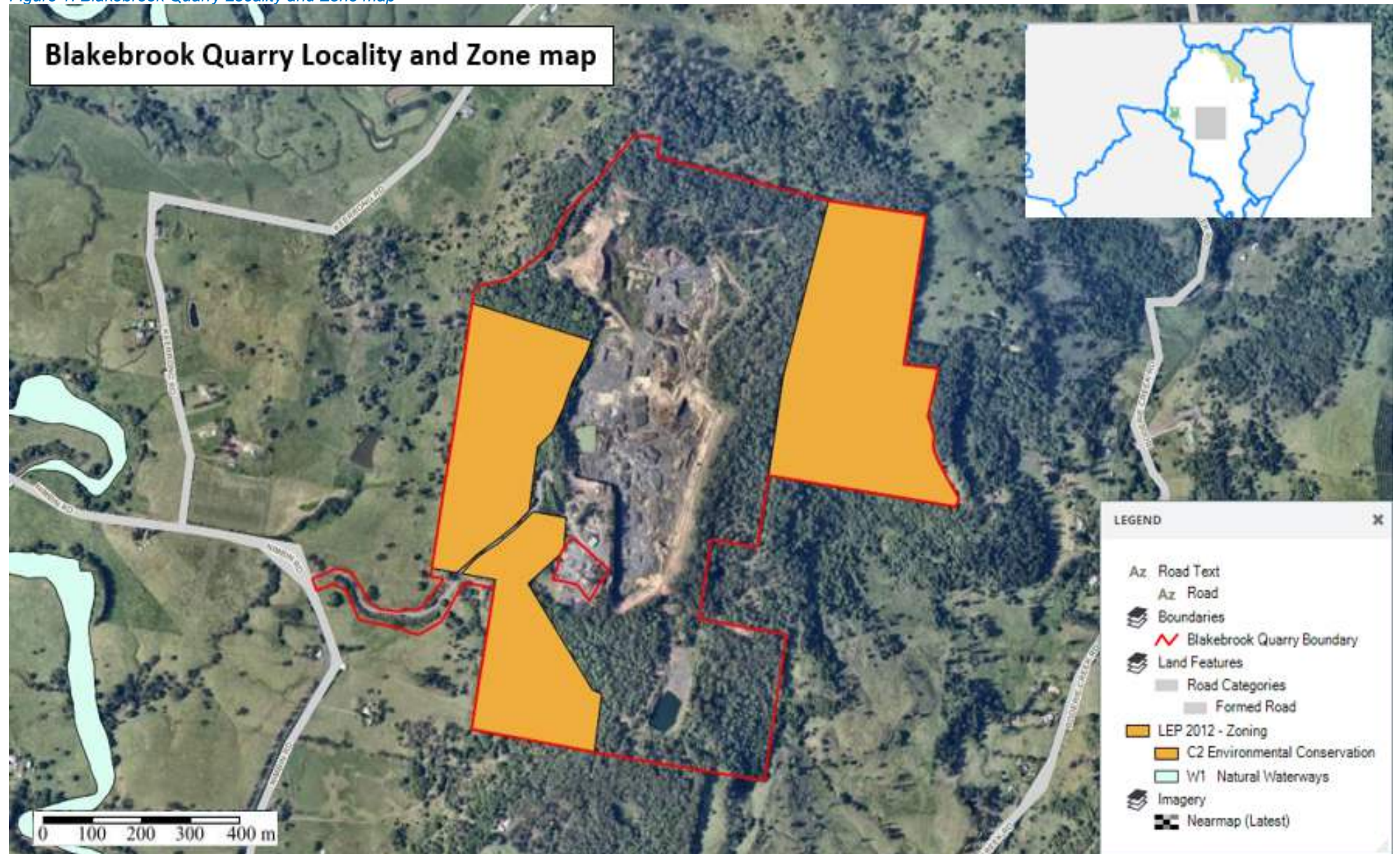
Figure 1: Blakebrook Quarry Locality and Zone map
