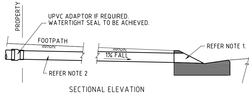
LAYBACK KERB
