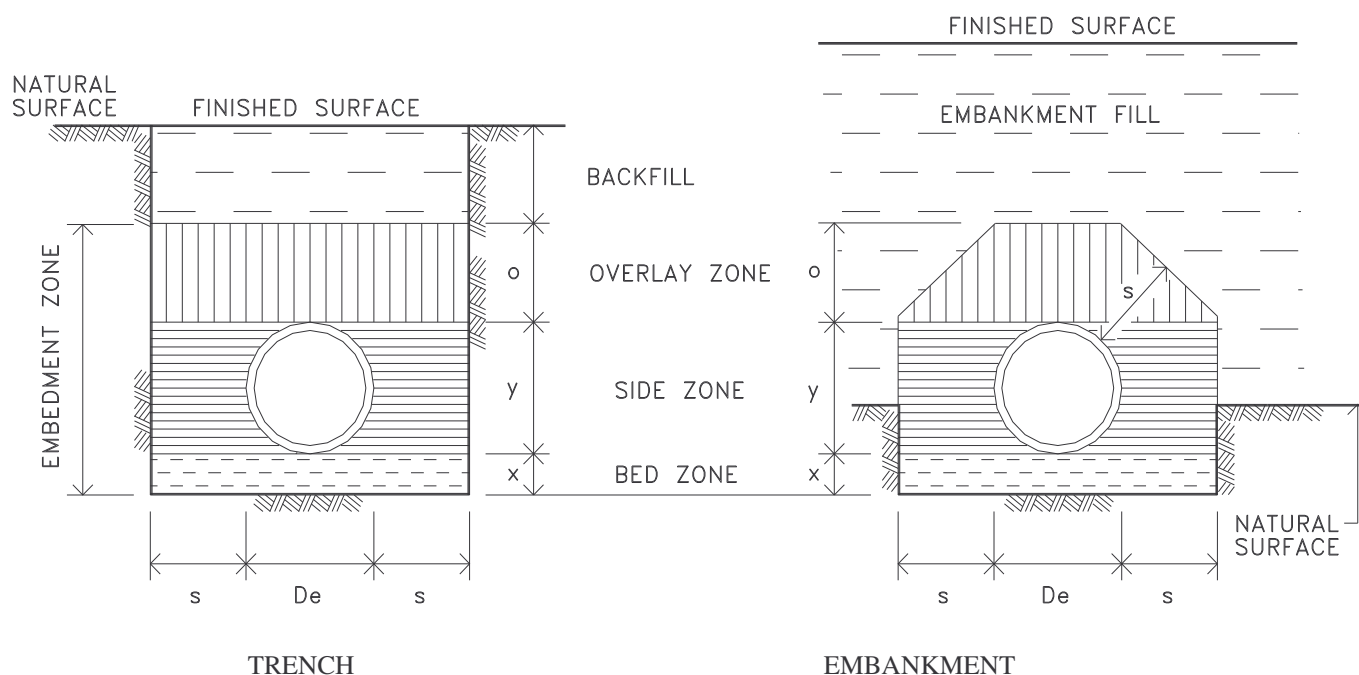
Figure C221.3 - Pipe Installation Conditions
